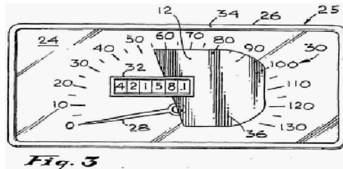
Figure 3 illustrates the speedometer display and colored plate combination of Evans. The colored plate 12 of Evans is a fixed structure integrally attached to
